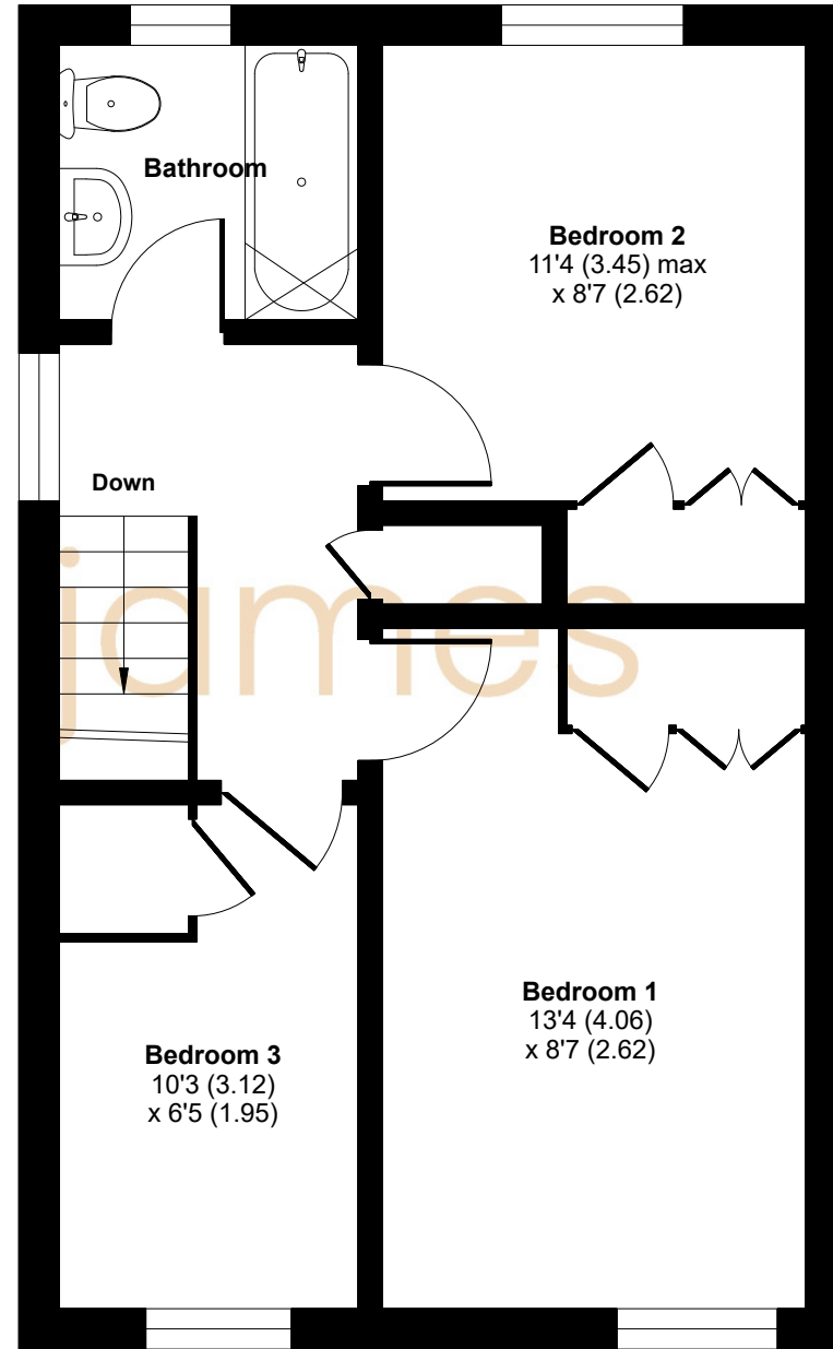
FIRST FLOOR
